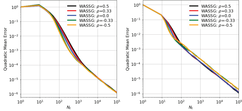
(A) Linear regression: Time-varying mini-batches with \{C_\rho = 8, \beta = 1/3\} (B) Geometric median: Time-varying mini-batches with \{C_\rho = 8, \beta = 1/3\}
